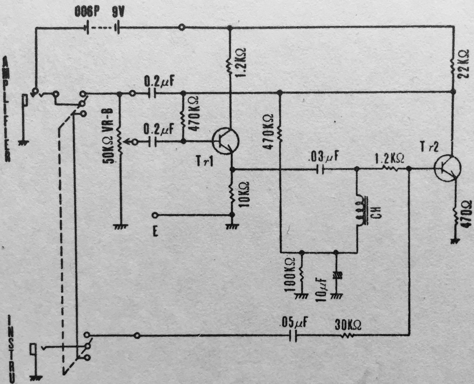
WT - 1 DIAGRAM
