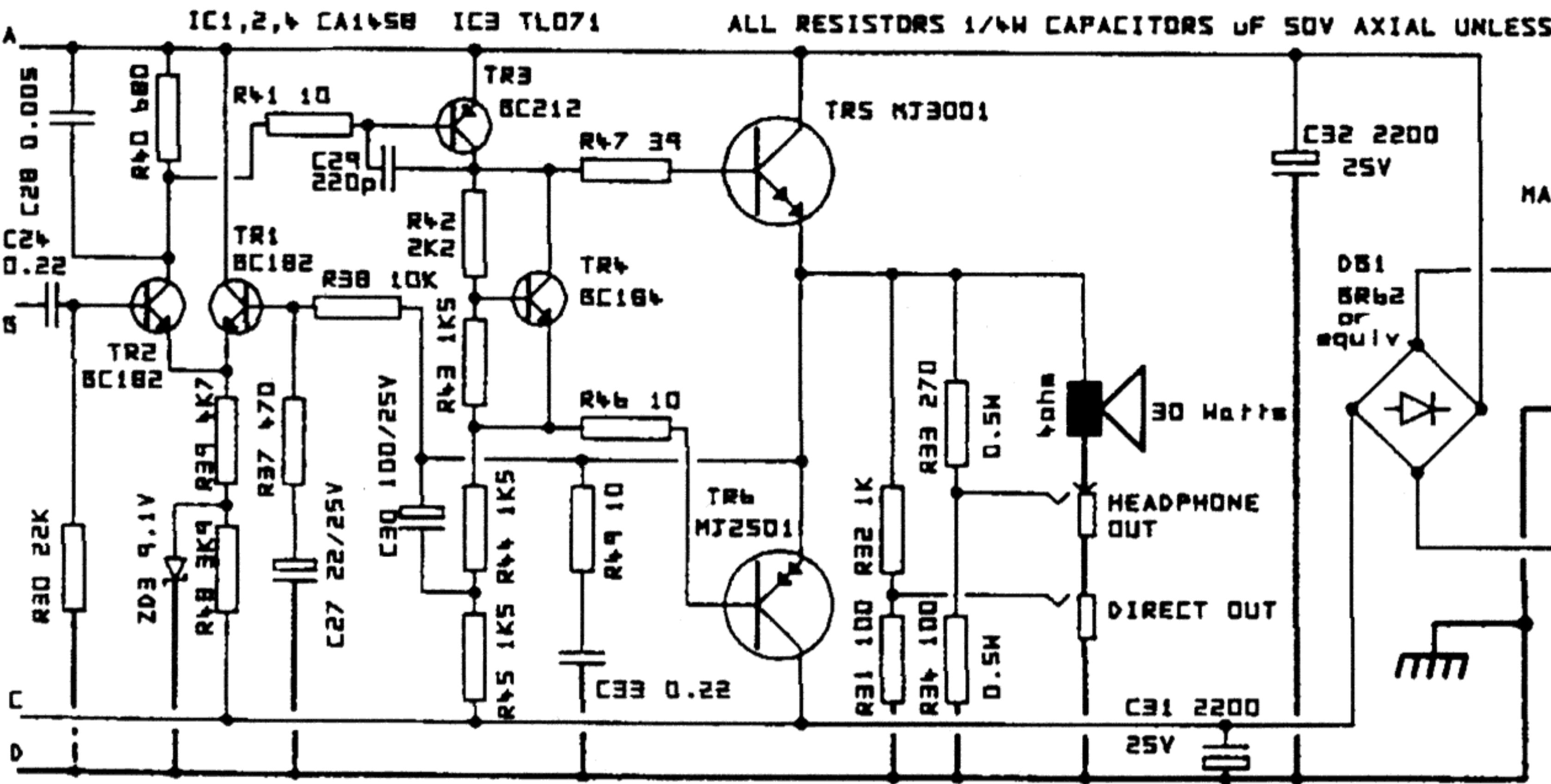
MARSHALL MODEL 5203 SCHEMATIC DIAGRAM
