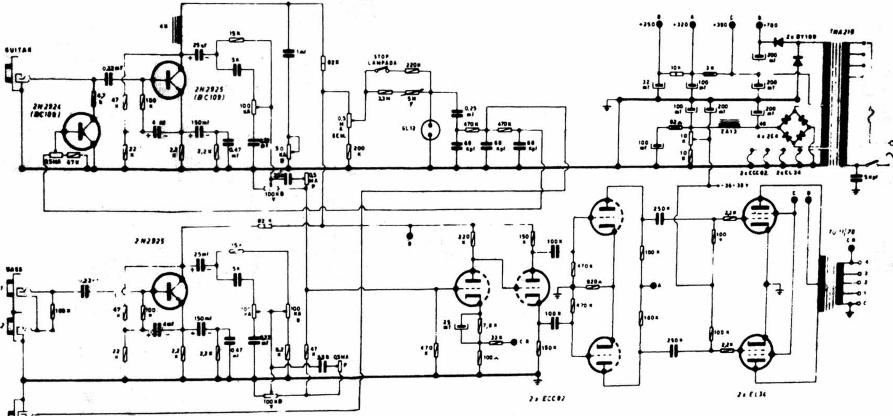
schema amplificatore PROFESSIONAL transistoro
