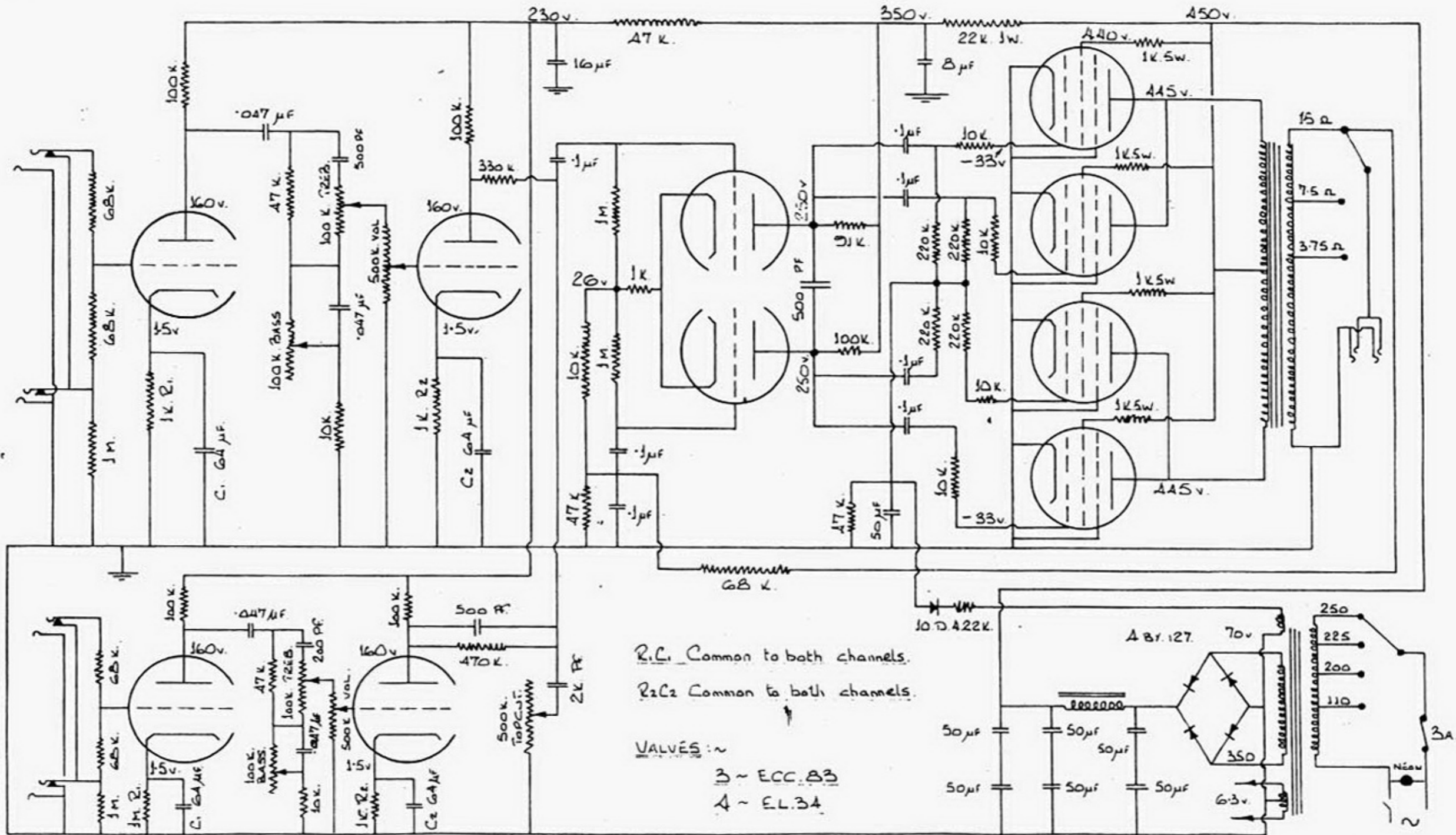
"CARLSBRO SOUND EQUIPMENT." (All voltages reference only) CS. 100.P.T.C.
