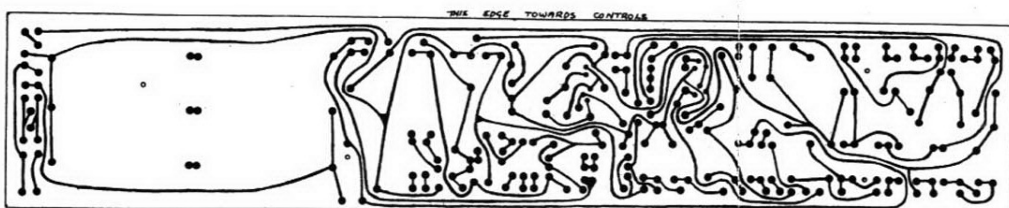
VIEW OF PRINTED CIRCUIT BOARD FROM COMPONENT SIDE
