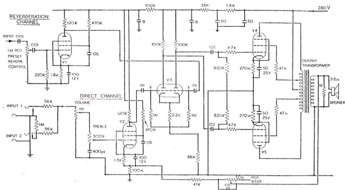
BIRD 15 WATT GUITAR AMPLIFIER "GOLDEN EAGLE"
