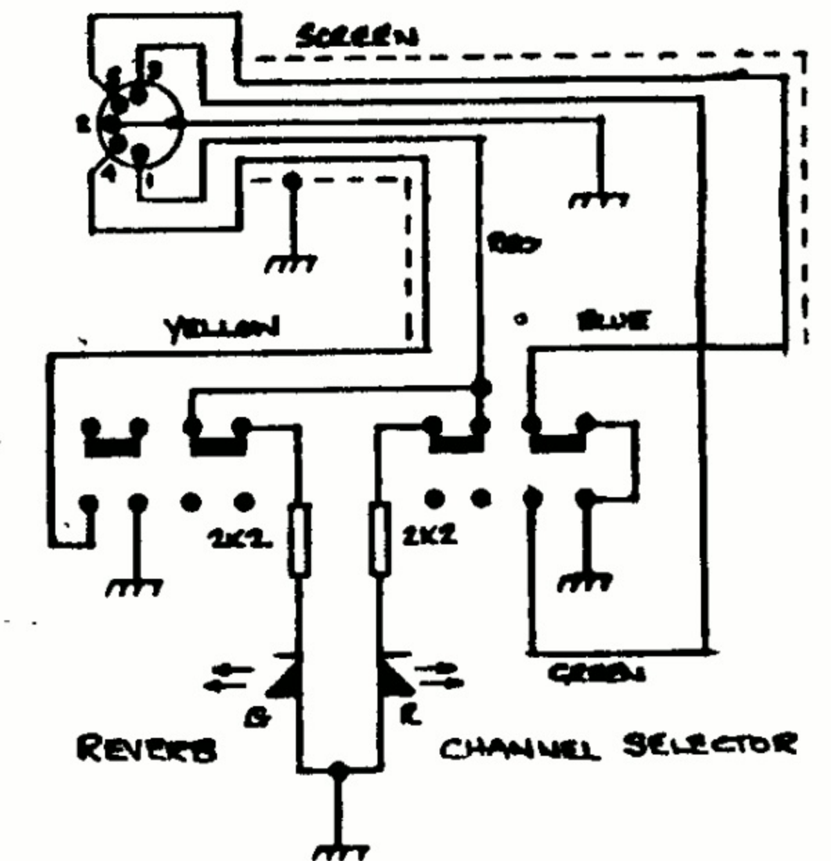
FOOT SWITCH SCHEMATIC
